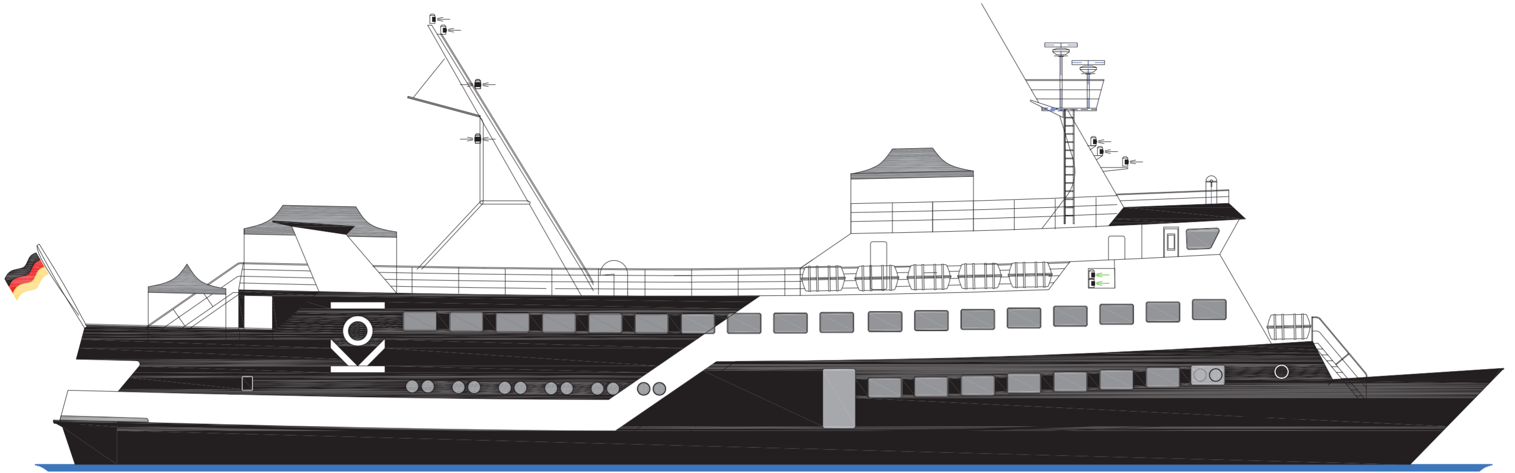
OPEN-AIR-DECK
