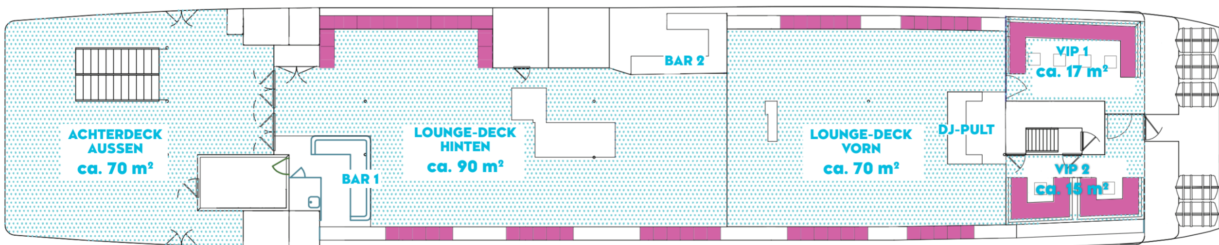
LOUNGE-DECK
